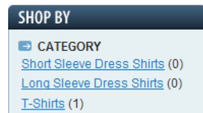
Figure 3: Layered Navigation
